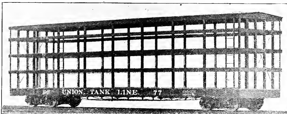
Fig. 15. BARREL CAR. UNION TANK LINE. Length, 51 ft. Capacity, 432 barrels, or 40,000 lbs.
